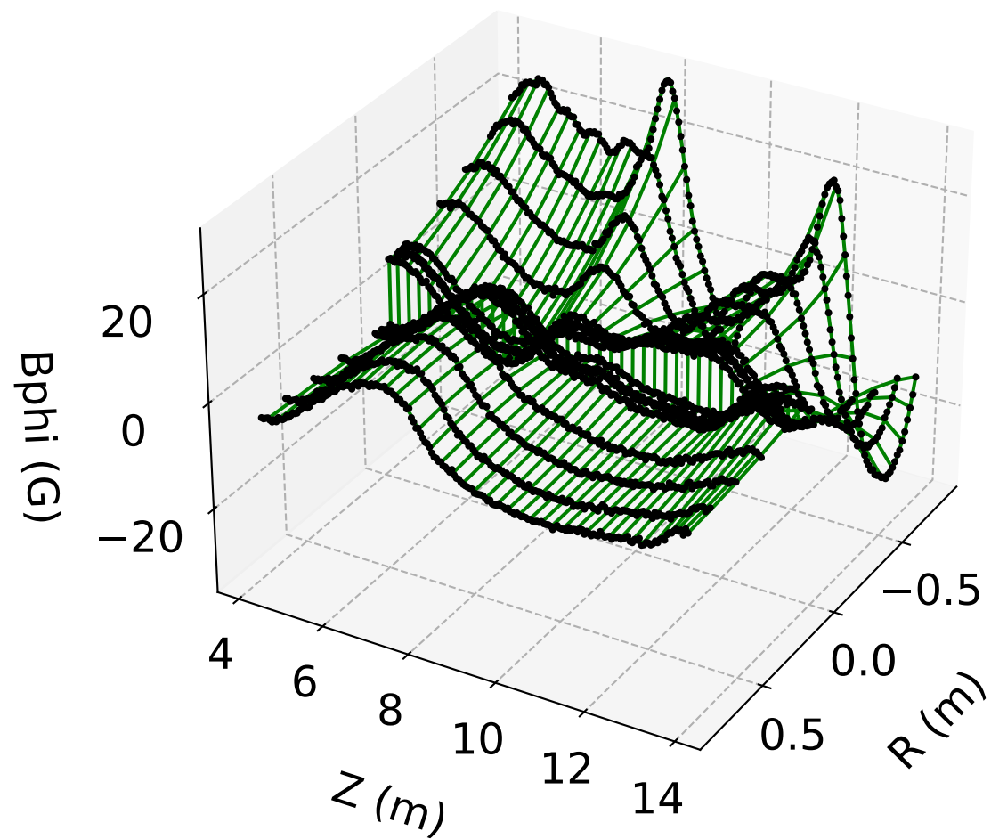
B_\phi vs. r, z ( \phi = 0 ) Full Model (#1)
