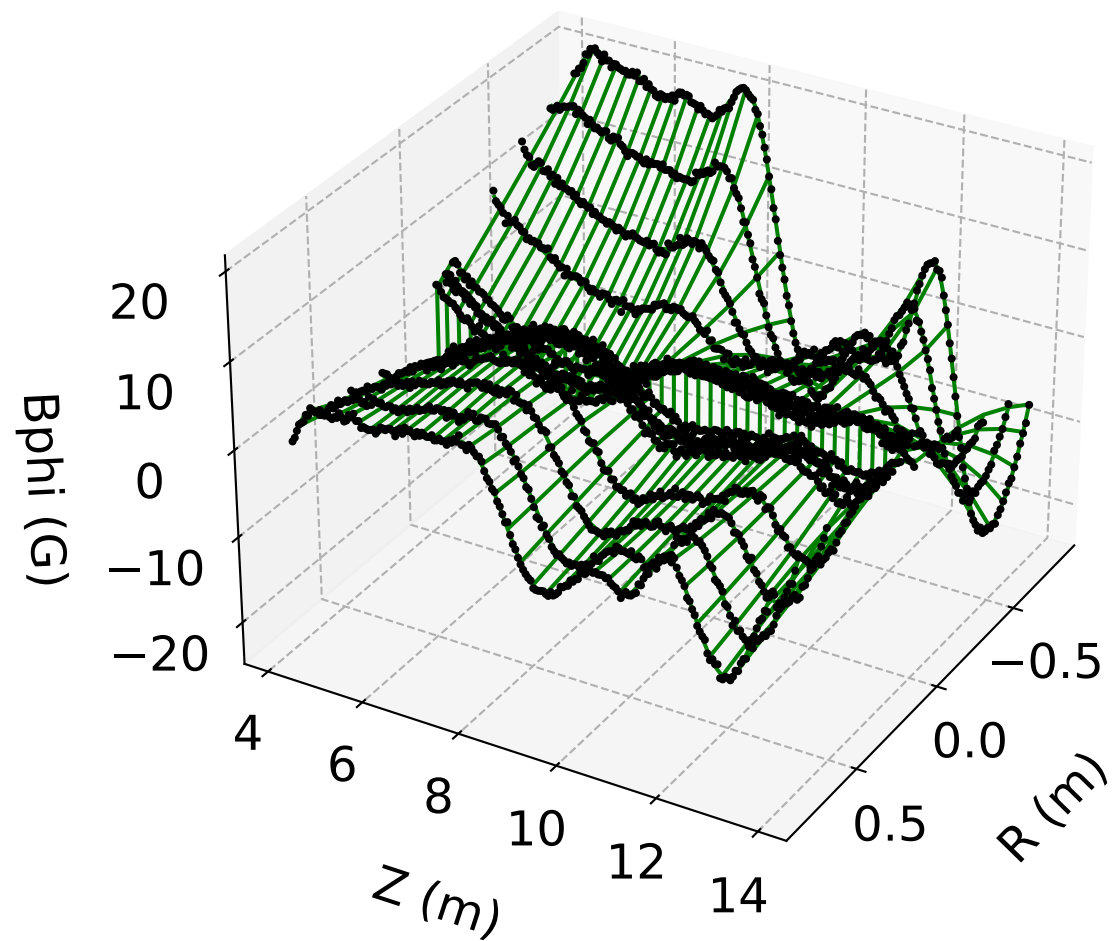
B_\phi vs. r, z ( \phi = 0 ) LSQ Refit (#1)
