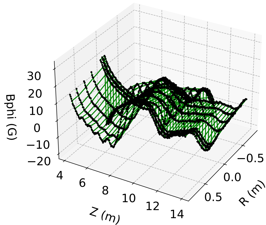
B_\phi vs. r, z ( \phi = \pi/2 ) Full Model (#1)
