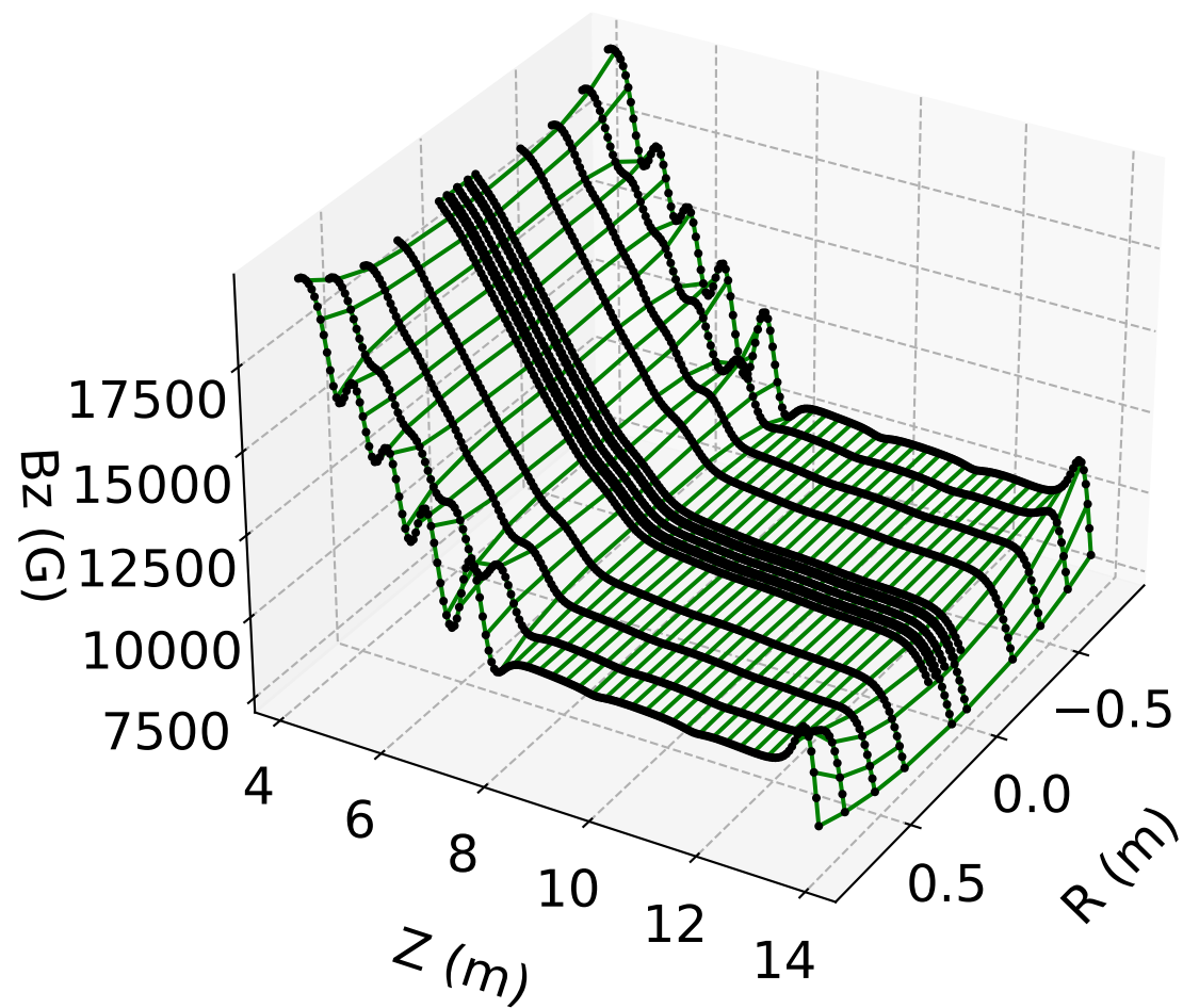
B_z vs. r, z ( \phi = 0 ) Full Model (#1)
