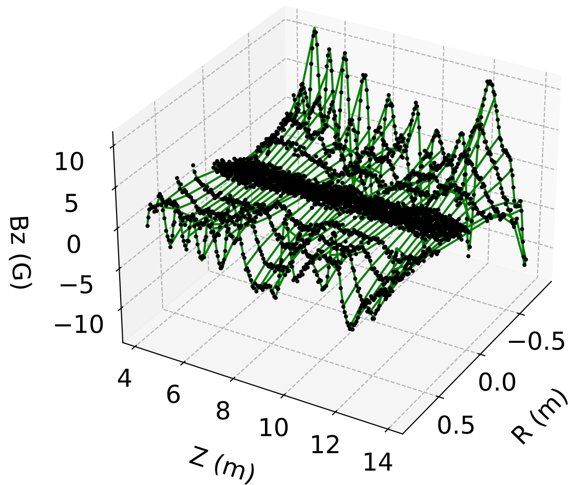
B_z vs. r, z ( \phi = 0 ) PINN Model (#1)
