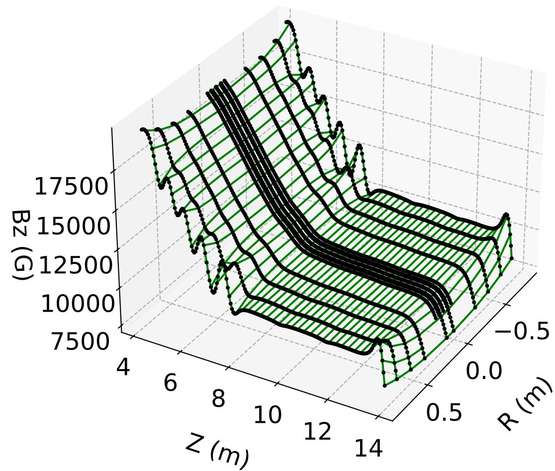
B_z vs. r, z ( \phi = \pi/2 ) Full Model (#1)
