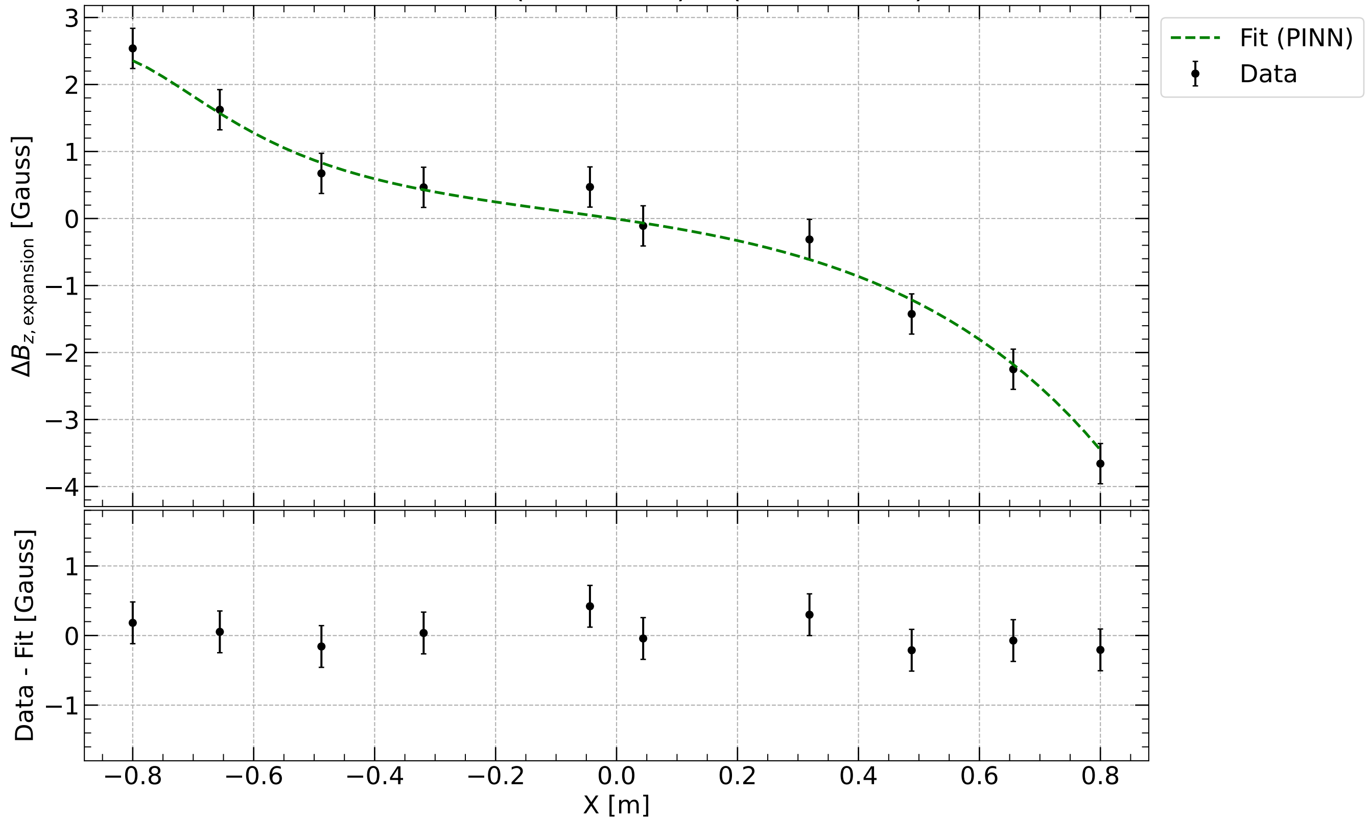
PINN Results: (Y==0.0 m) & (Z==8.40 m)
