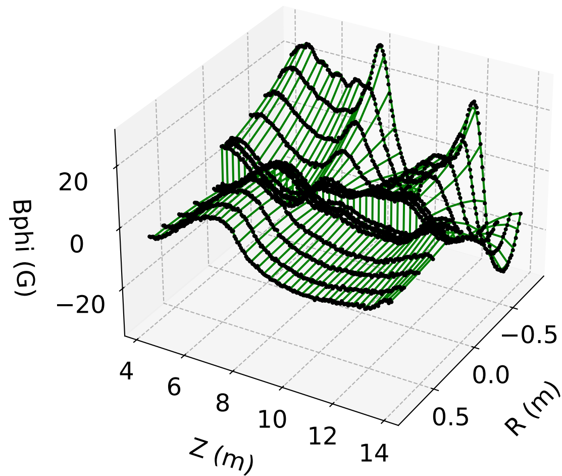
B_\phi vs. r, z ( \phi = 0 ) Full Model (#2)
