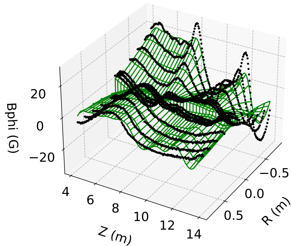
B_\phi vs. r, z ( \phi = 0 ) LSQ Model (#2)
