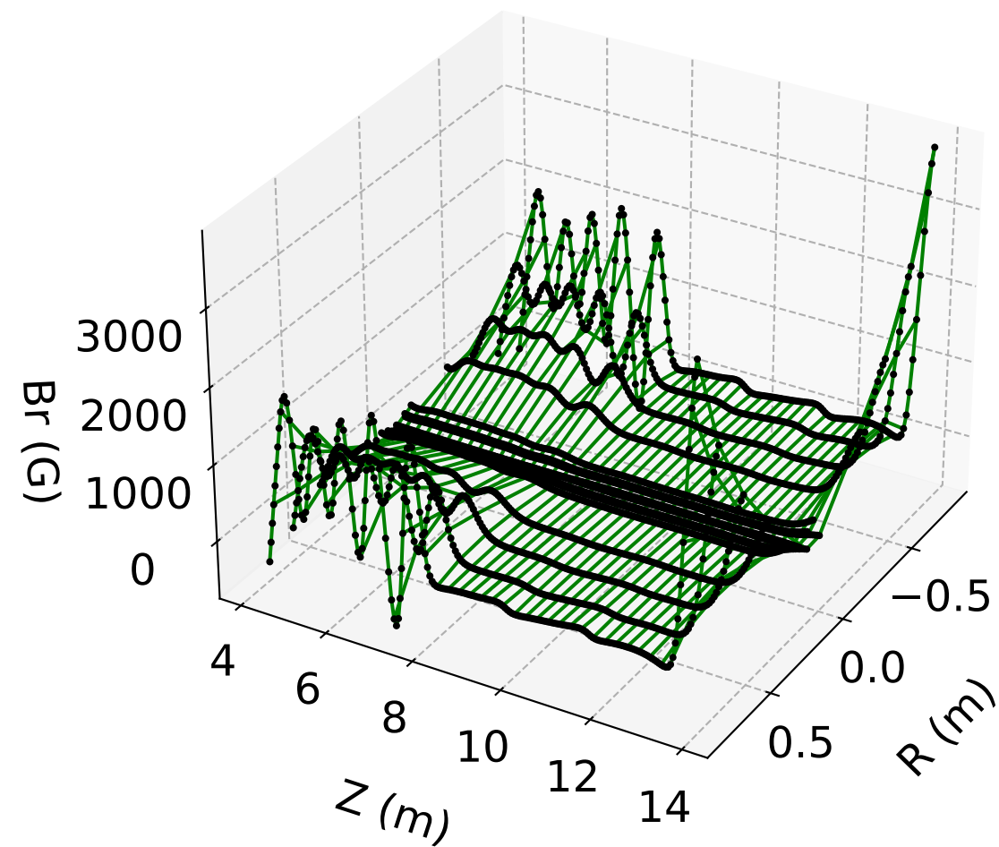
B_r vs. r, z ( \phi = 0 ) LSQ Model (#2)
