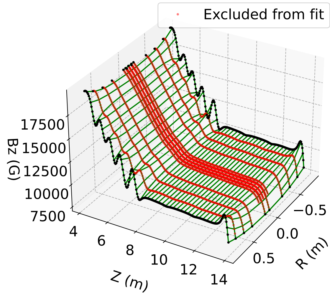
B_z vs. r, z ( \phi = 0 ) LSQ Model (#3)
