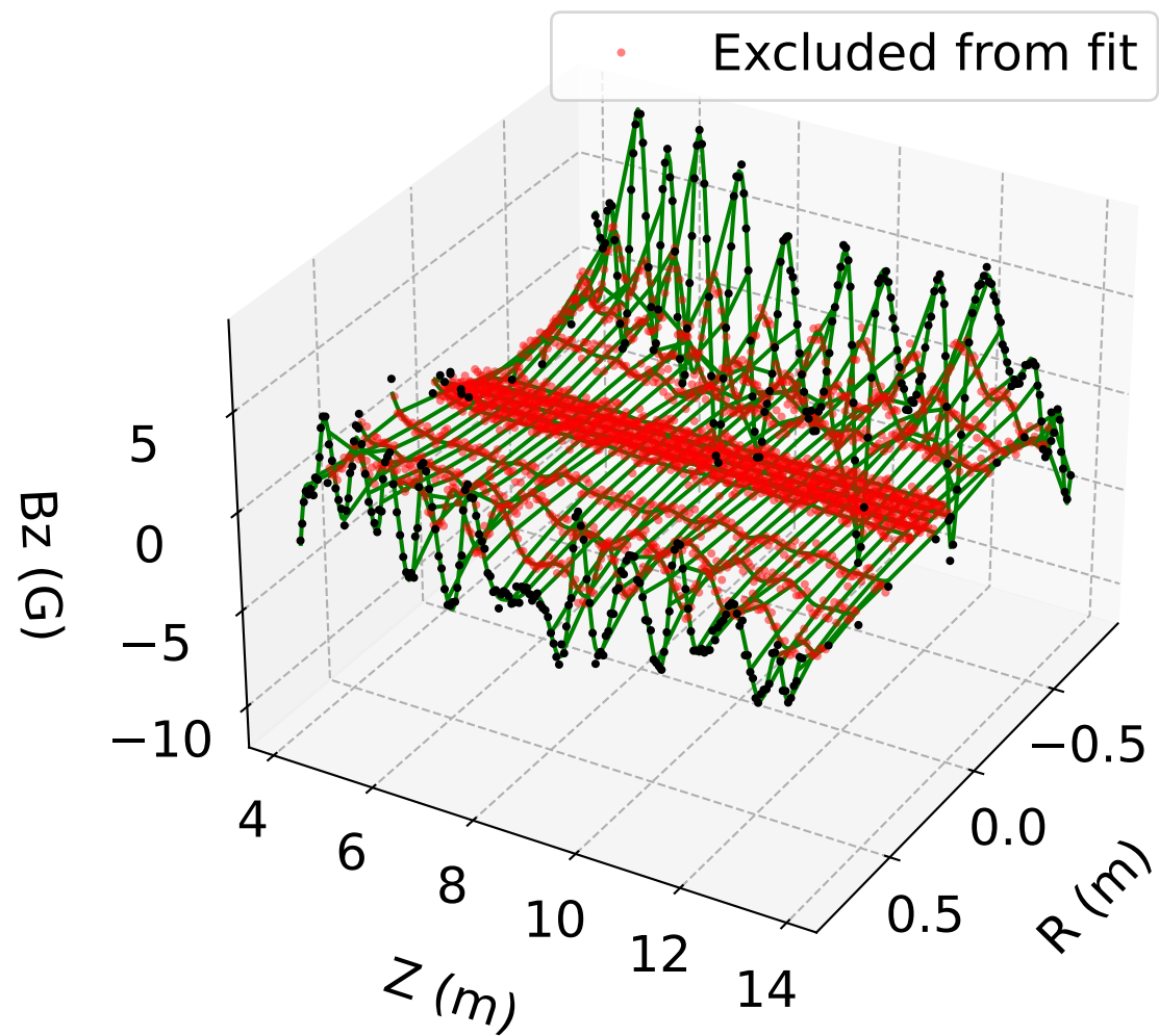
B_z vs. r, z ( \phi = 0 ) PINN Model (#3)
