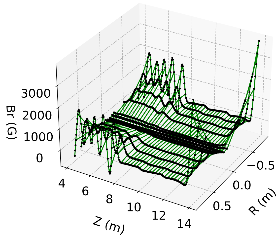
B_r vs. r, z ( \phi = 0 ) LSQ Model (#4)
