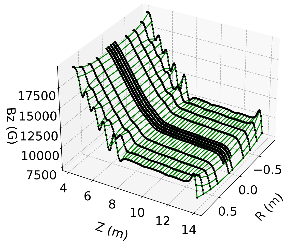
B_z vs. r, z ( \phi = 0 ) LSQ Model (#4)
