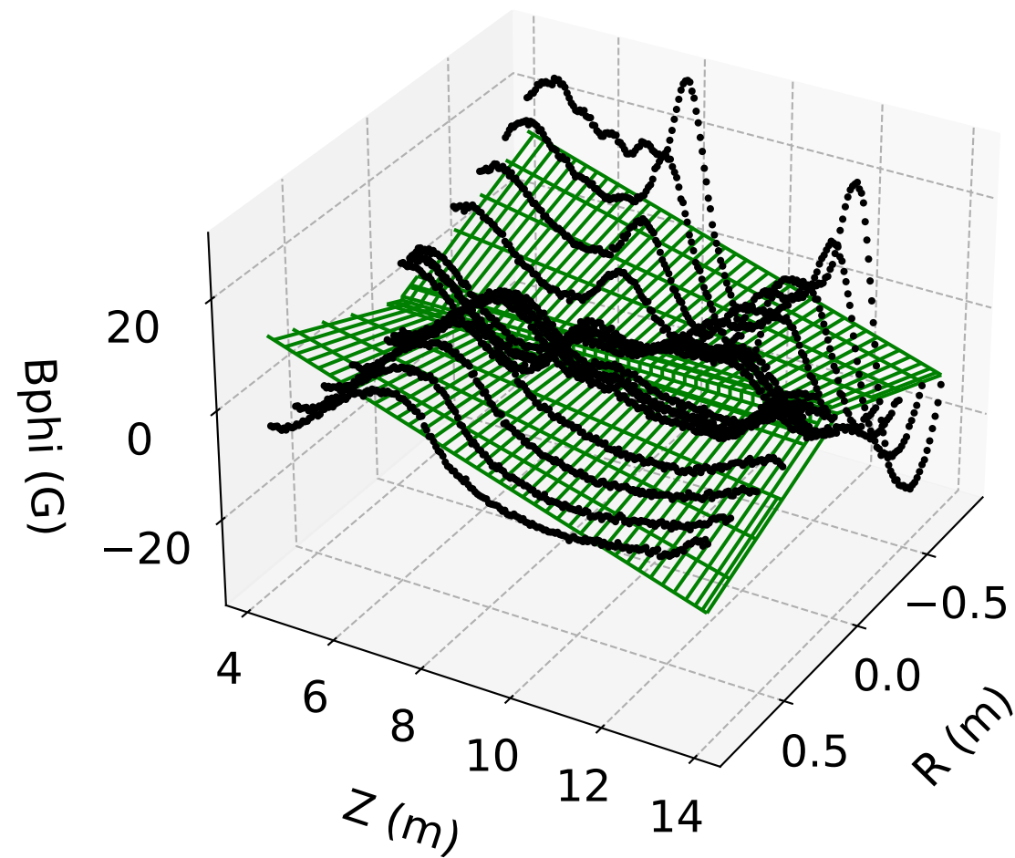
B_\phi vs. r, z ( \phi = 0 ) LSQ Model (#5)
