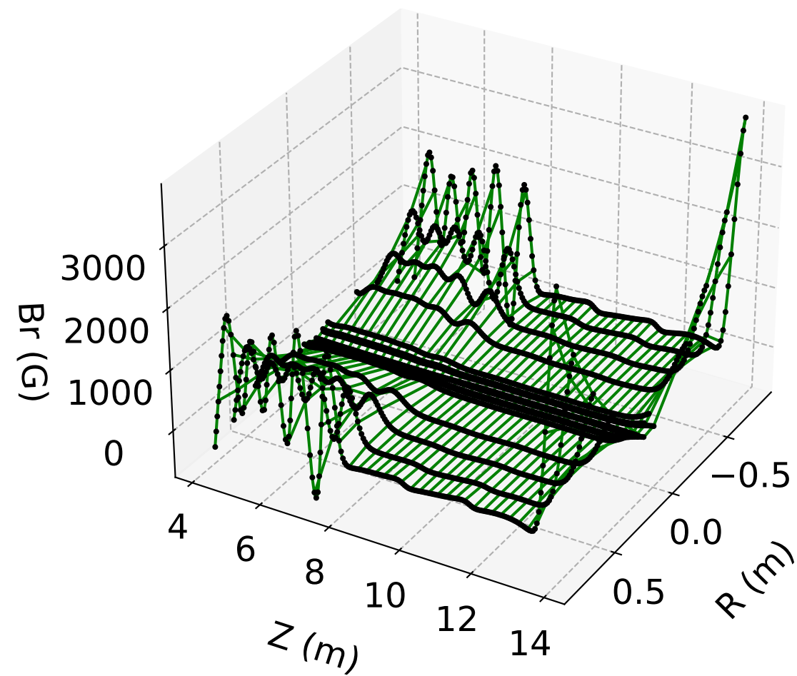
B_r vs. r, z ( \phi = 0 ) LSQ Model (#5)
