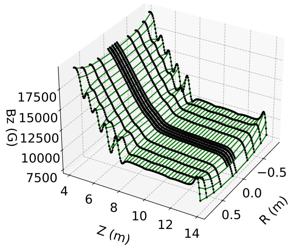
B_z vs. r, z ( \phi = 0 ) Full Model (#5)
