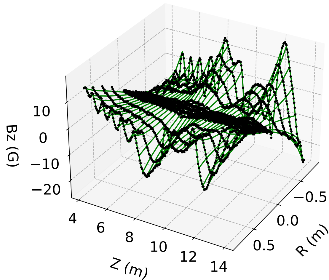
B_z vs. r, z ( \phi = 0 ) PINN Model (#5)
