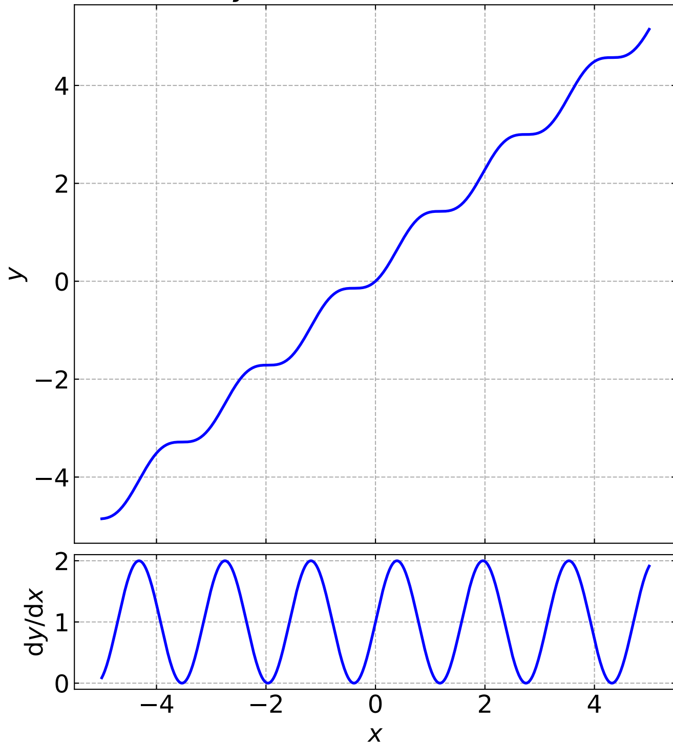
Snake: y = x + 1/a \cdot \sin^2(ax) ; a = 2
