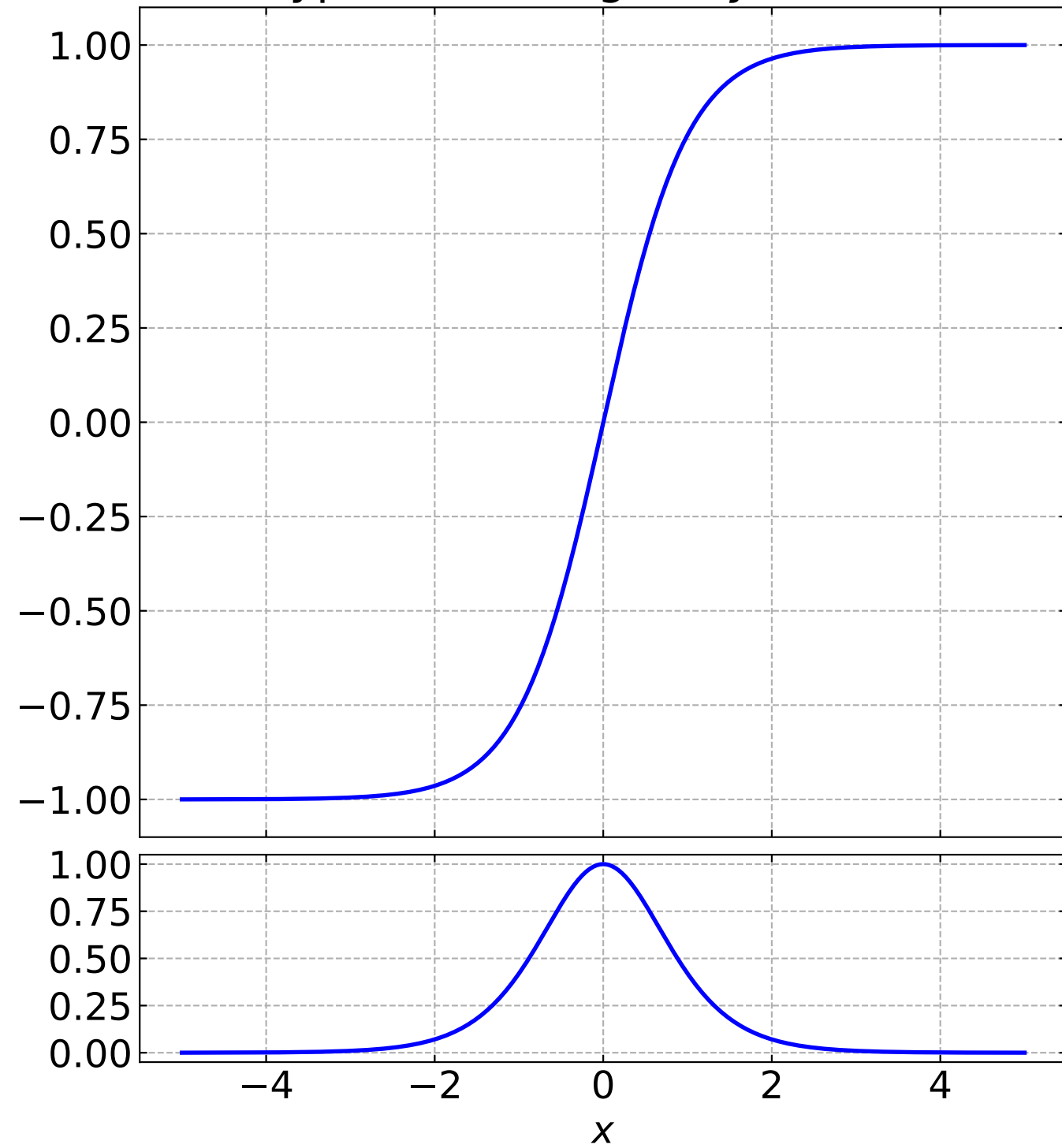
Hyperbolic Tangent: y = \tanh x
