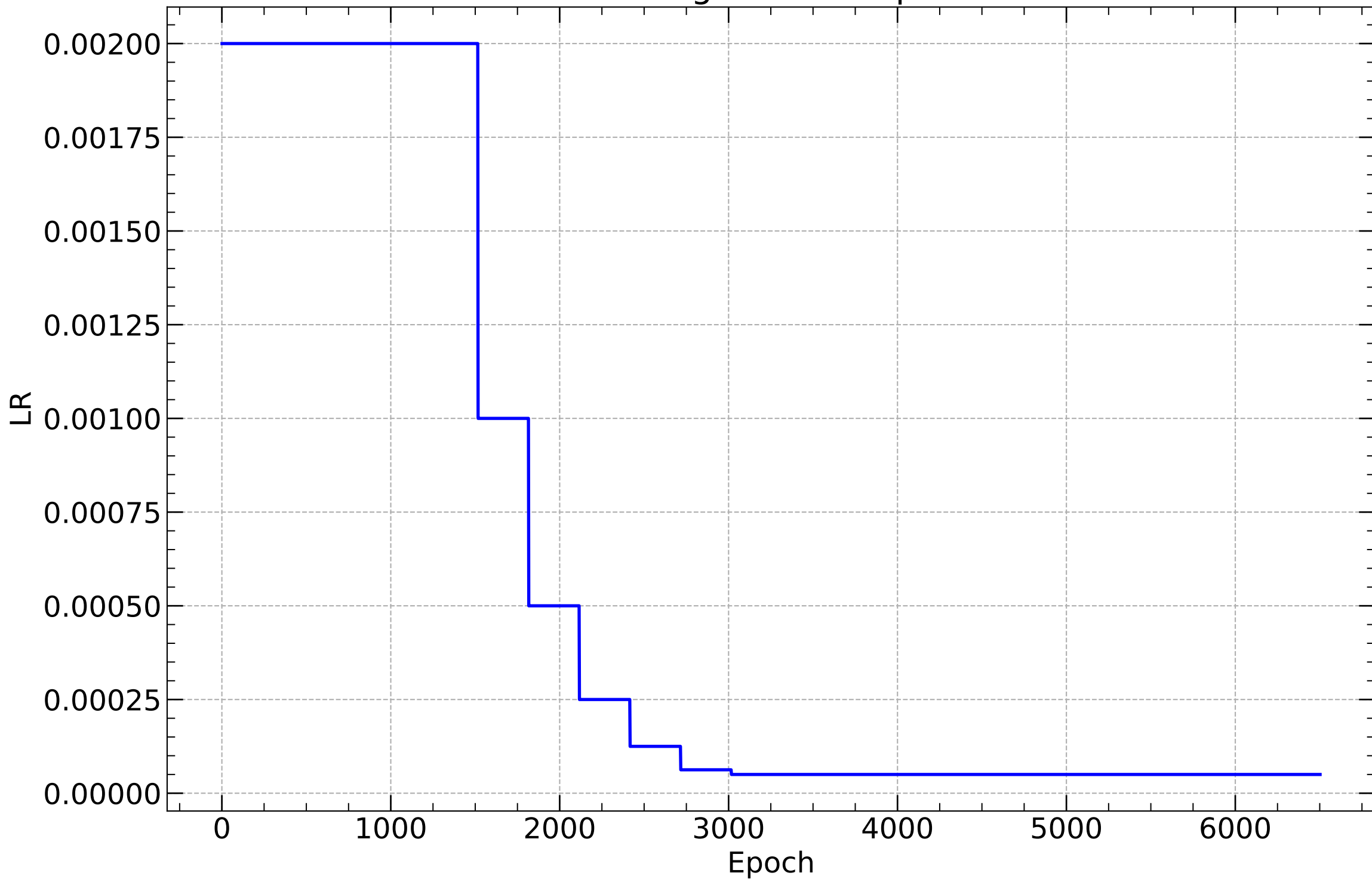
Learning Rate vs. Epoch
