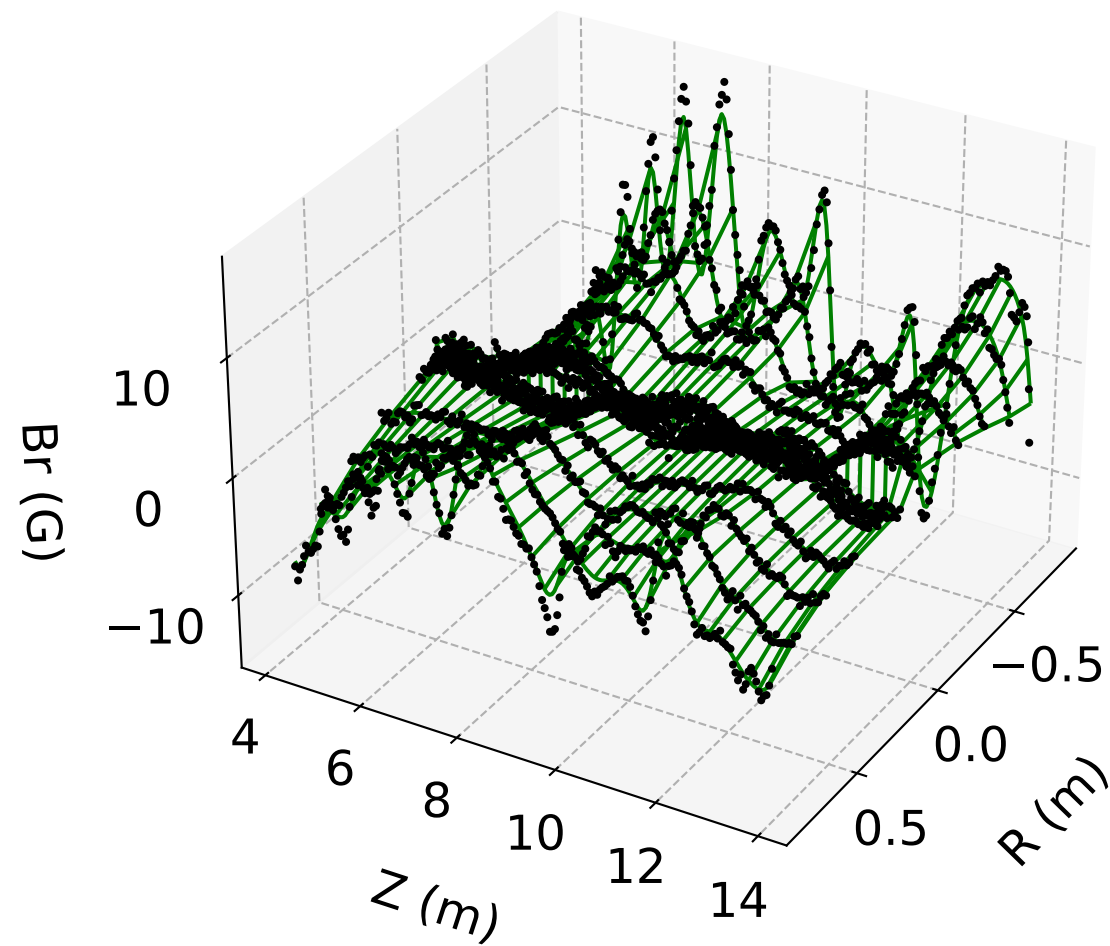
B_r vs. r, z ( \phi = 0 ) PINN Model (#2)
