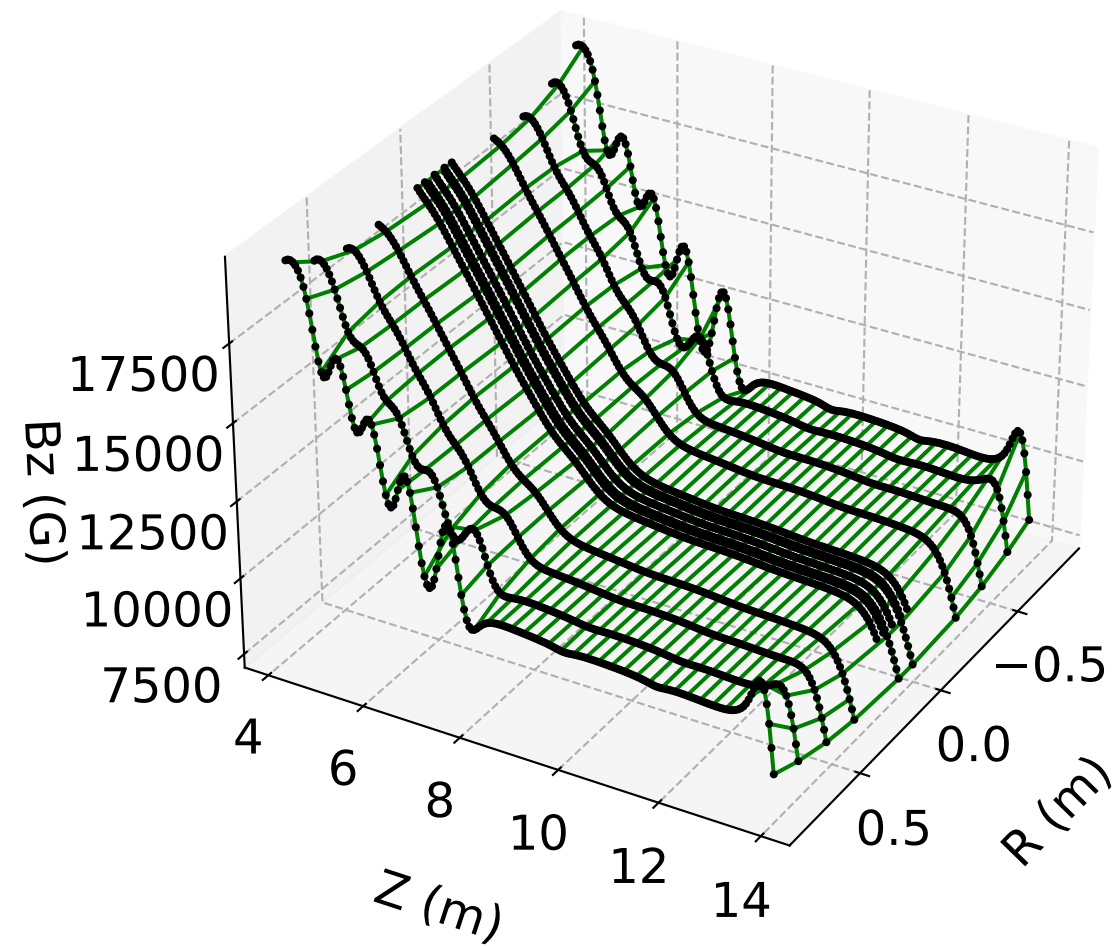
B_z vs. r, z ( \phi = 0 ) Full Model (#2)
