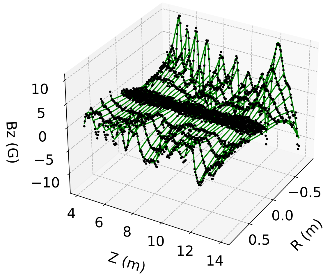
B_z vs. r, z ( \phi = 0 ) PINN Model (#2)
