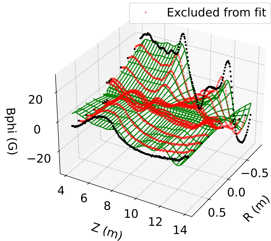
B_\phi vs. r, z ( \phi = 0 ) LSQ Model (#3)
