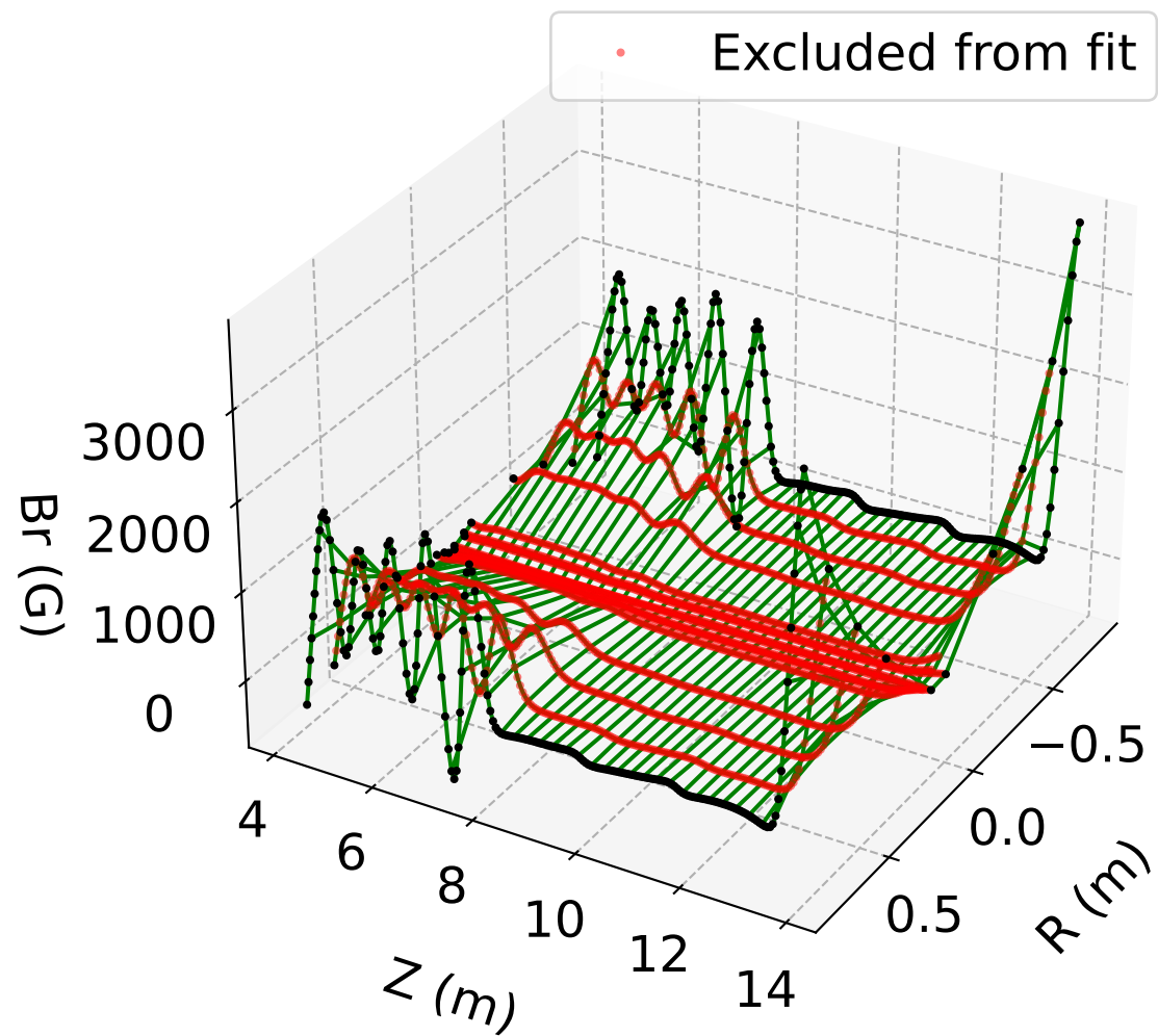
B_r vs. r, z ( \phi = 0 ) Full Model (#3)
