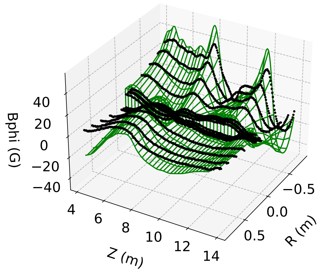
B_\phi vs. r, z ( \phi = 0 ) Full Model (#4)
