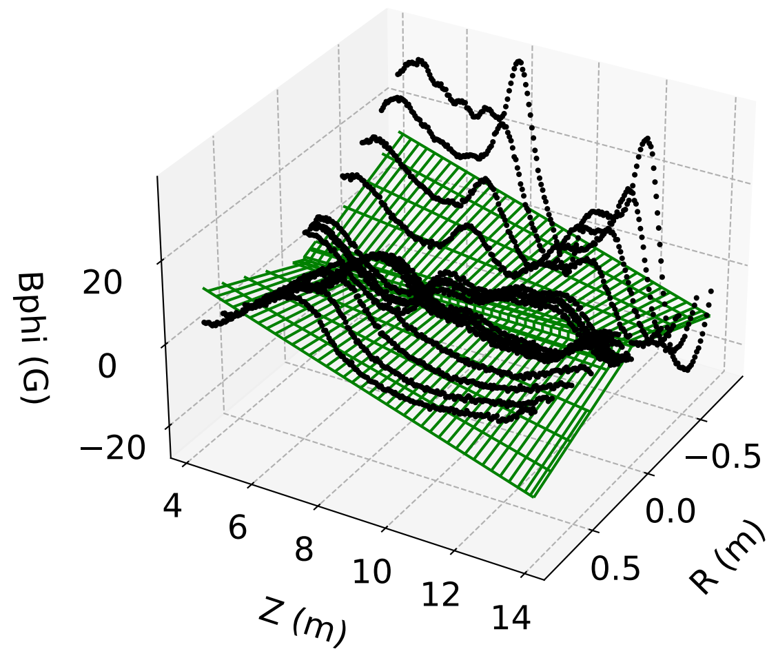
B_\phi vs. r, z ( \phi = 0 ) LSQ Model (#4)
