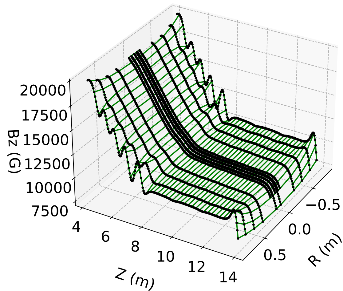
B_z vs. r, z ( \phi = 0 ) Full Model (#4)
