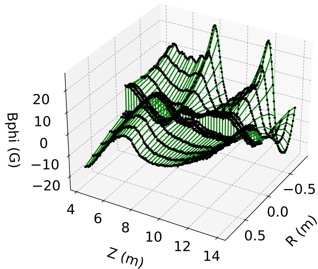
B_\phi vs. r, z ( \phi = 0 ) PINN Model (#5)
