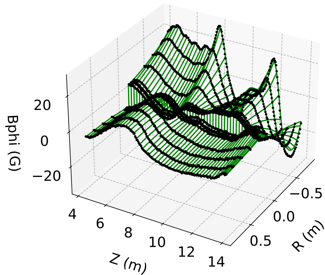
B_\phi vs. r, z ( \phi = 0 ) LSQ Model (#8)
