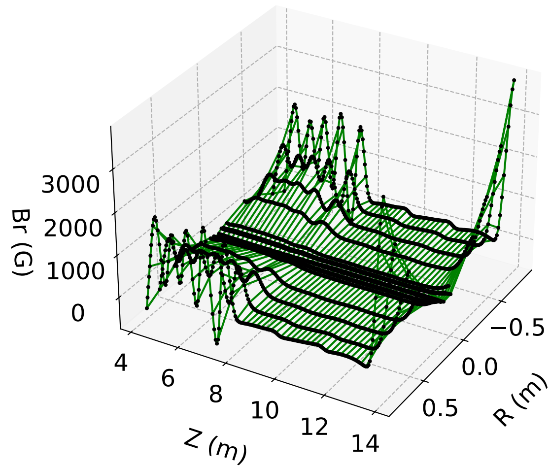
B_r vs. r, z ( \phi = 0 ) Full Model (#8)
