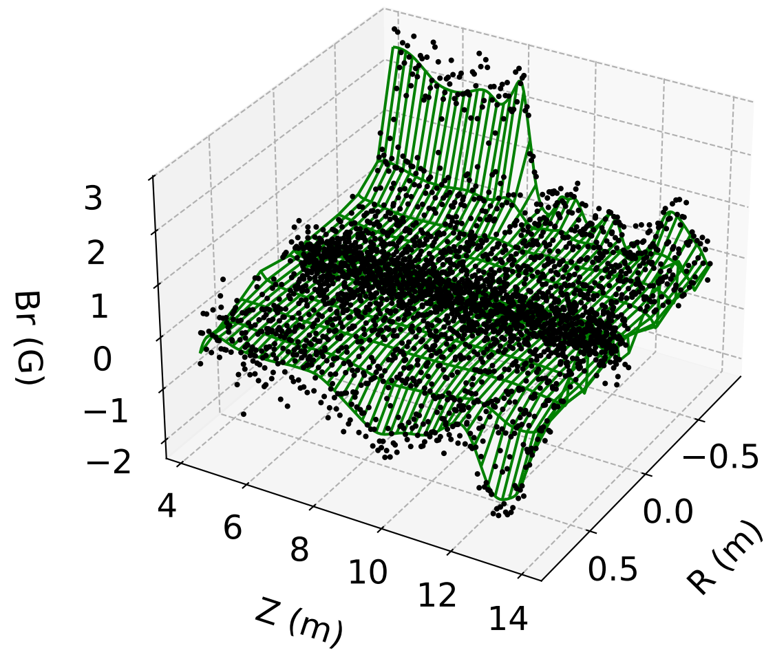
B_r vs. r, z ( \phi = 0 ) PINN Model (#8)
