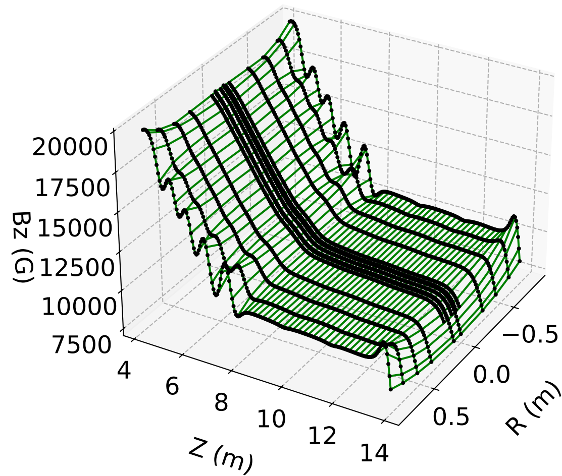
B_z vs. r, z ( \phi = 0 ) Full Model (#8)
