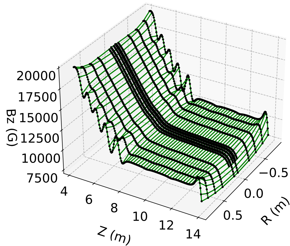
B_z vs. r, z ( \phi = 0 ) LSQ Model (#8)
