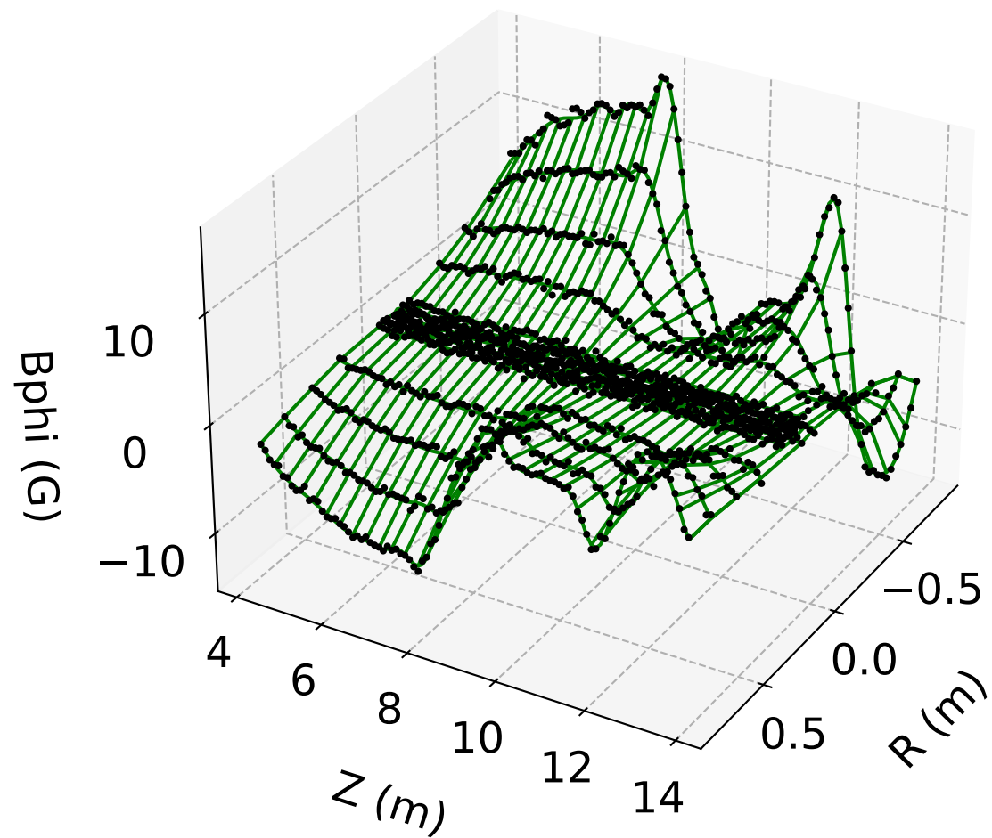
B_\phi vs. r, z ( \phi = 0 ) PINN Model (#9)
