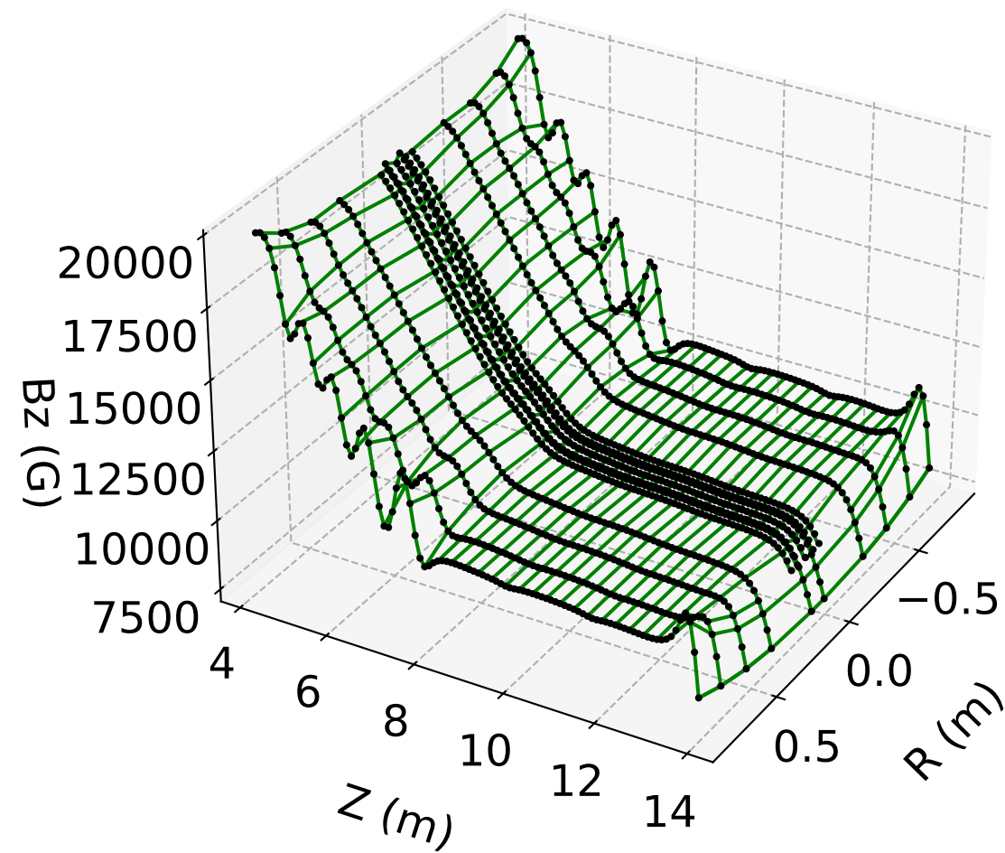
B_z vs. r, z ( \phi = 0 ) LSQ Model (#9)
