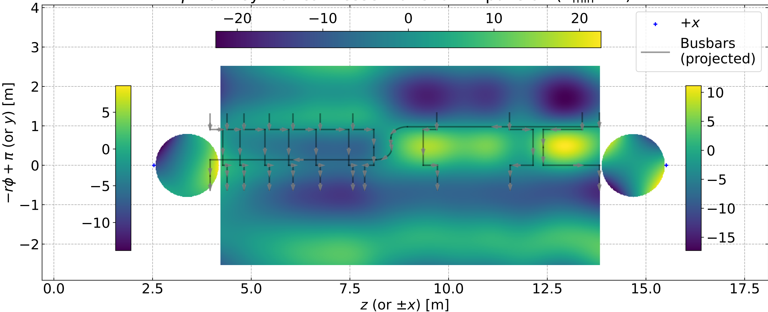
\phi from Cylindrical Bessel Function Expansion ( n_{\min} = 1 )
