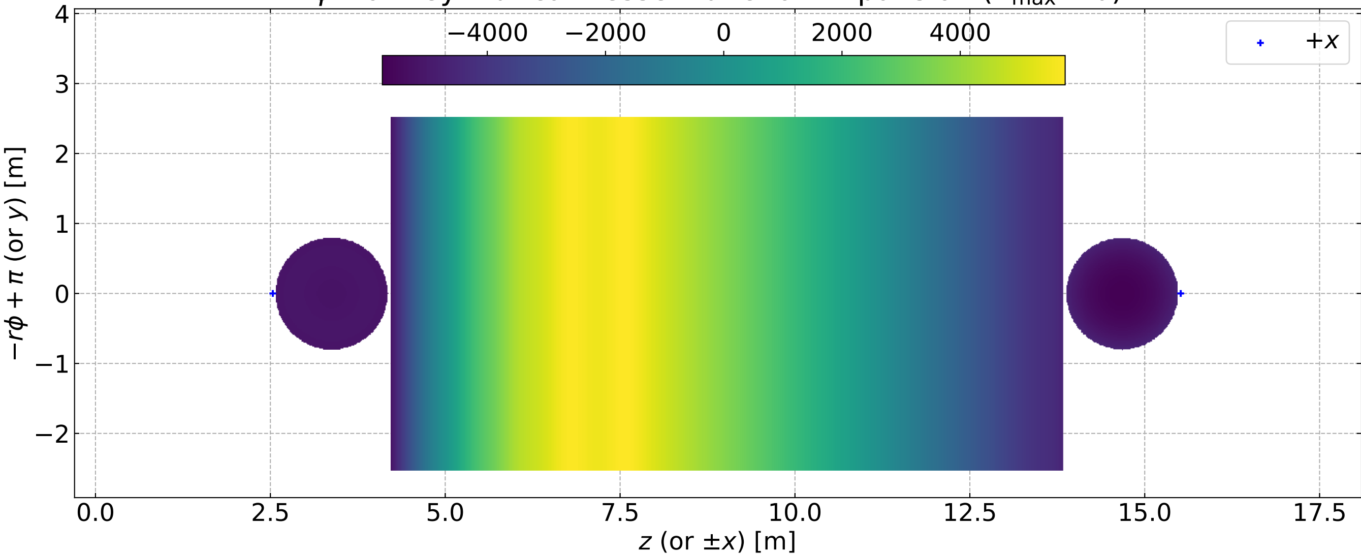
\phi from Cylindrical Bessel Function Expansion ( n_{\max} = 0 )
