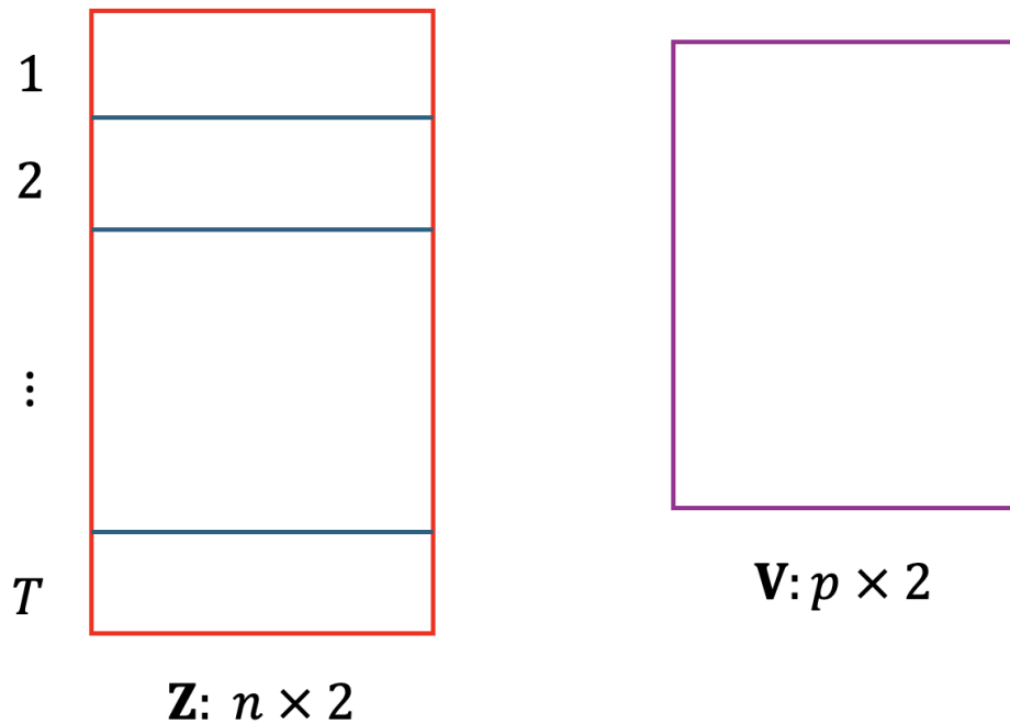
Figure 1: The fixed variable framework where the sample scores in matrix \mathbf{Z} are sliced according to the levels of the time variable T and the variable vectors in matrix \mathbf{V} remaining fixed.
