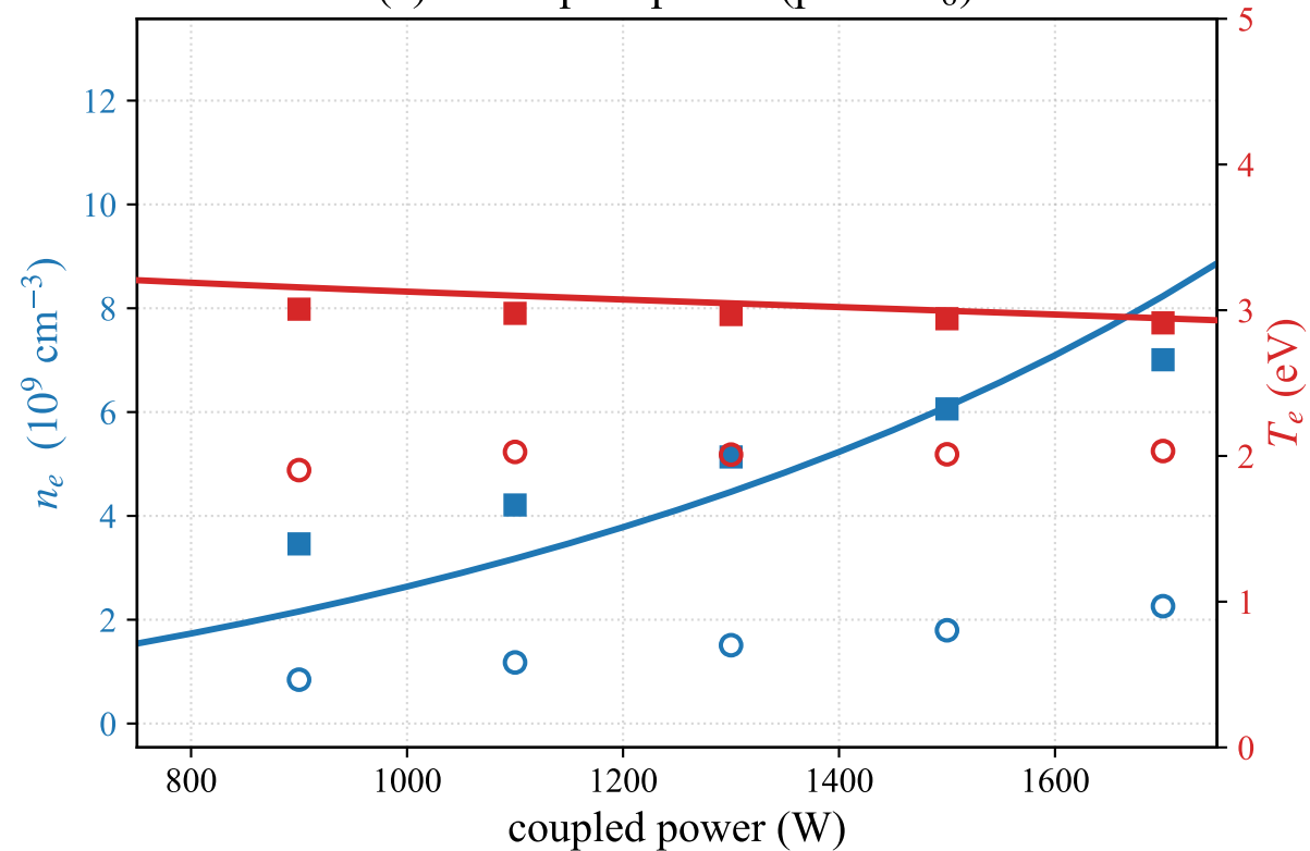
(a) vs coupled power (pure SF 6 )
