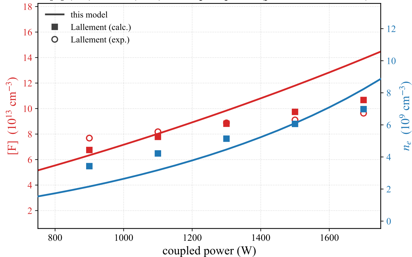
[F] (red) and n_e (blue) vs coupled power (pure SF 6 , 10 mTorr)
