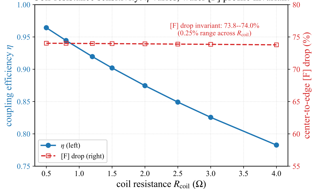
Coil-resistance sensitivity: \eta varies, wafer [F] profile invariant
