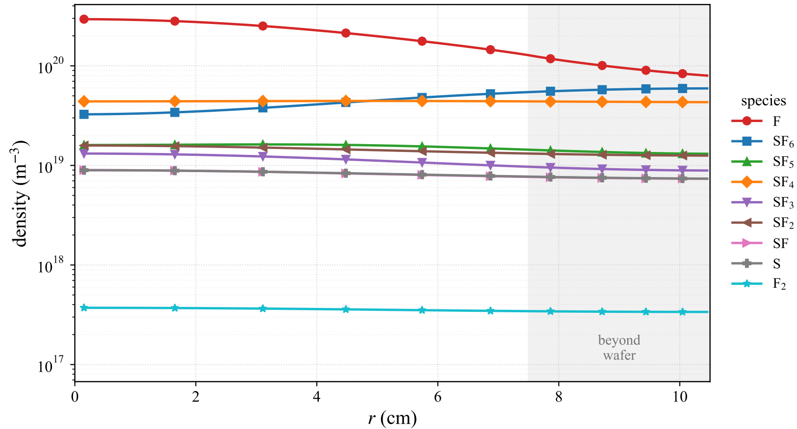
Wafer-plane radial profiles (70% SF 6 /30% Ar)
