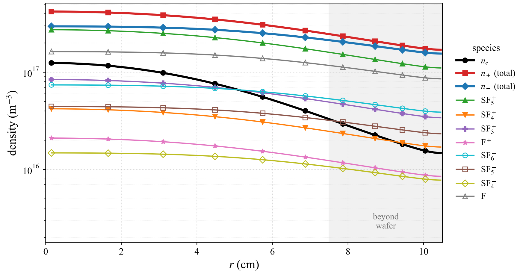
Wafer-plane charged-species profiles (70% SF 6 /30% Ar)
