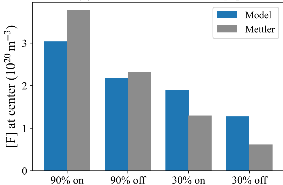
(b) Absolute wafer-center [F]
