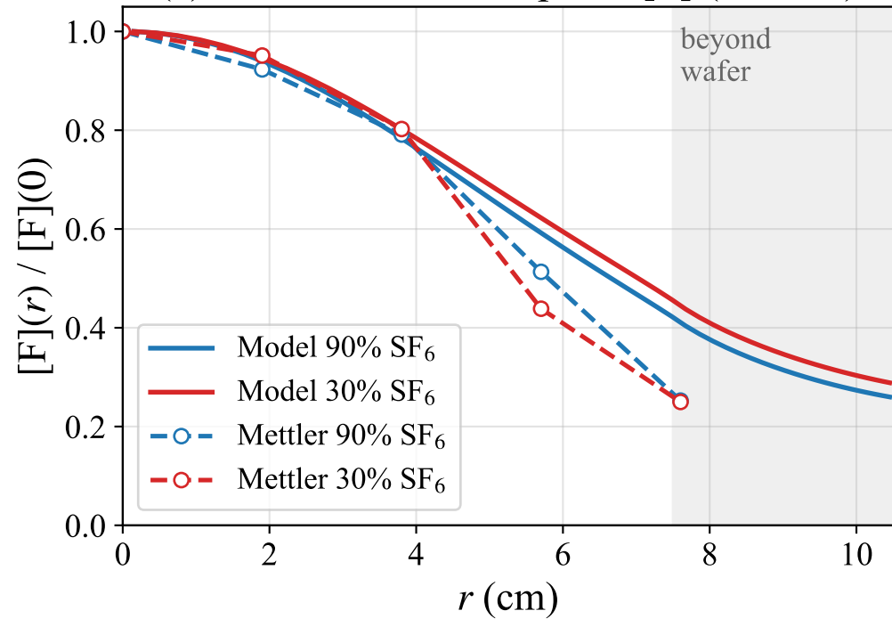
(a) Normalized wafer-plane [F] (bias-on)
