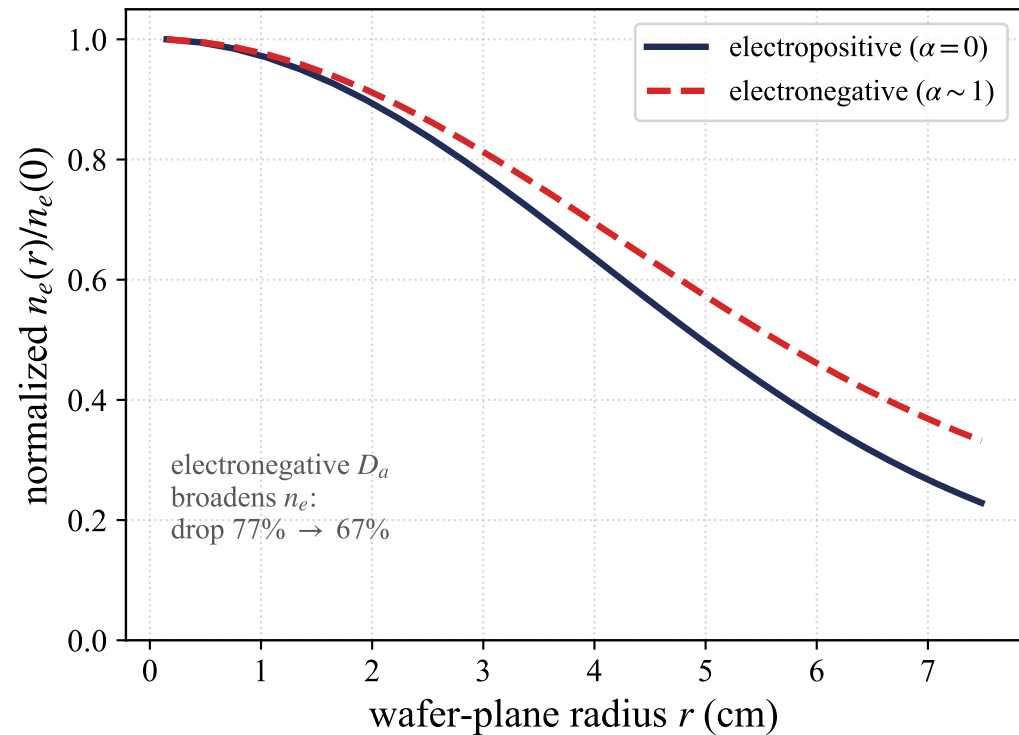
(a) electron density n_e(r) — set by D_a
