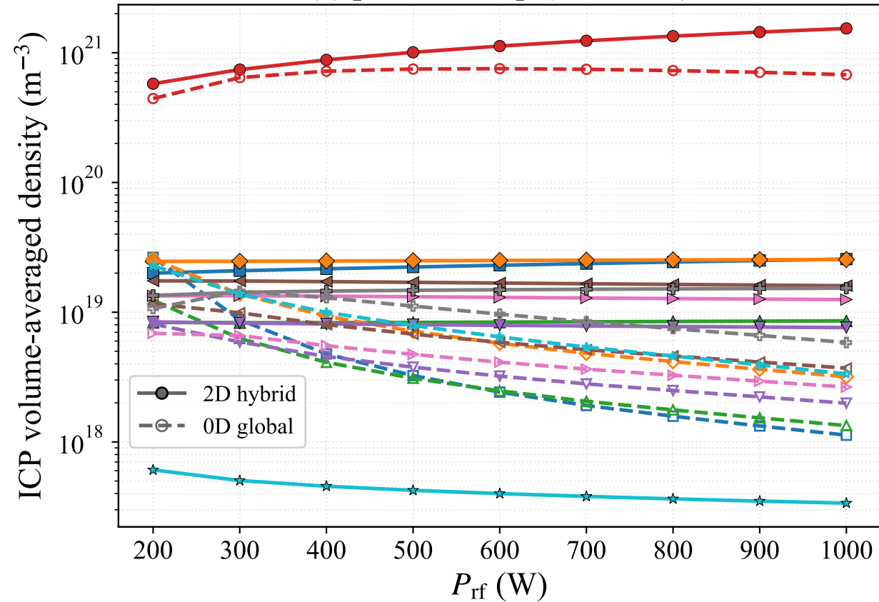
(a) power sweep (10 mTorr)
