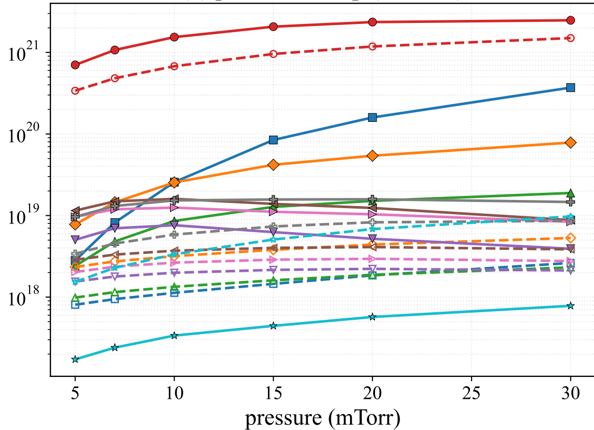
(b) pressure sweep (1000 W)
