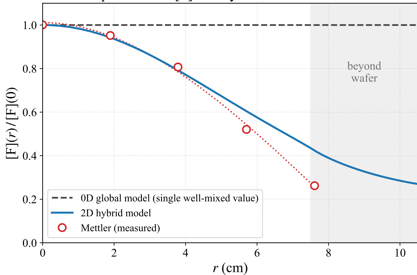
Wafer-plane radial [F]: 2D hybrid vs 0D vs measurement
