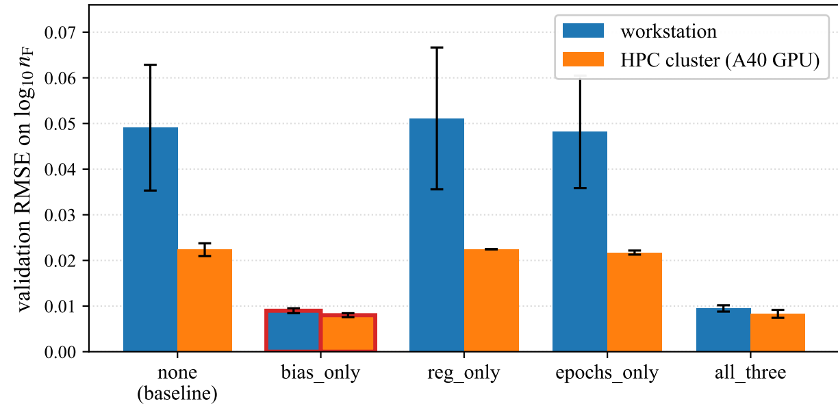
Training-recipe ablation (3 seeds, common schedule, two platforms)
