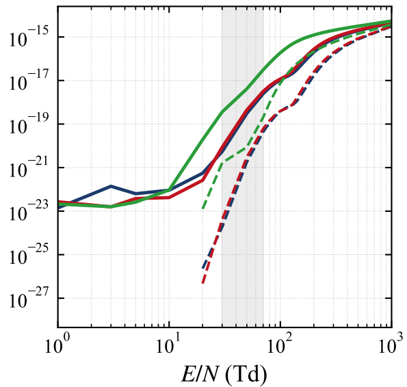
Dissociation
