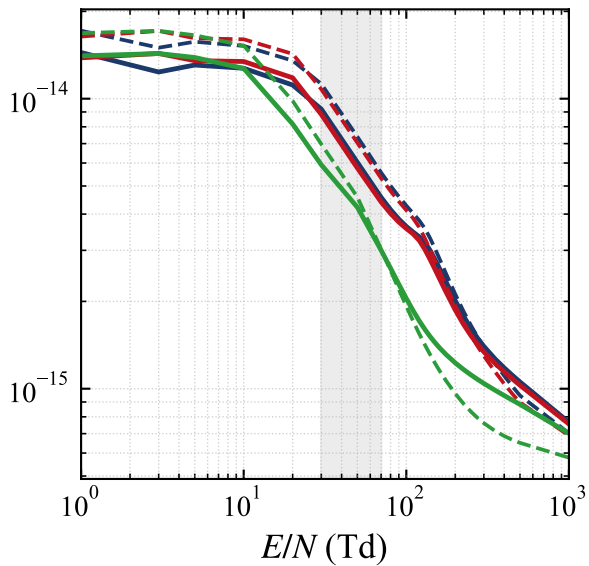
Attachment
